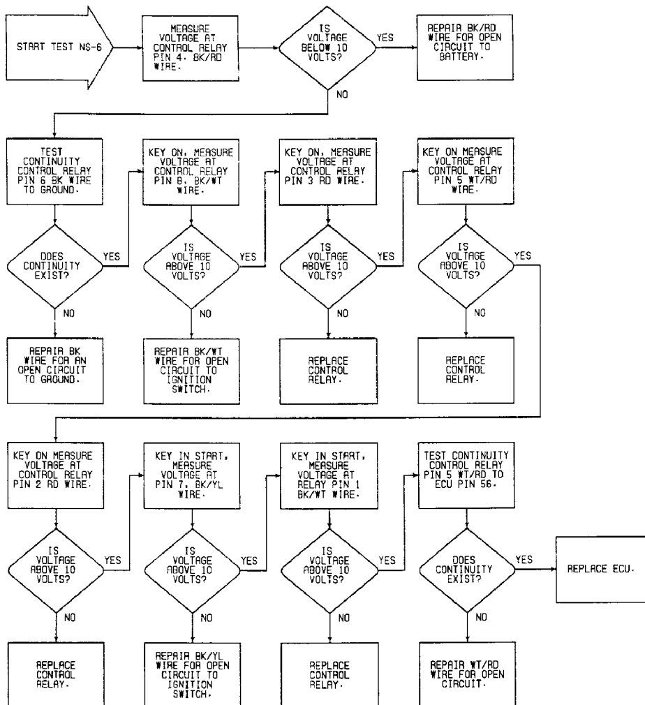
Fig. 22: No Start Test 6 Flow Chart Testing Control Relay
