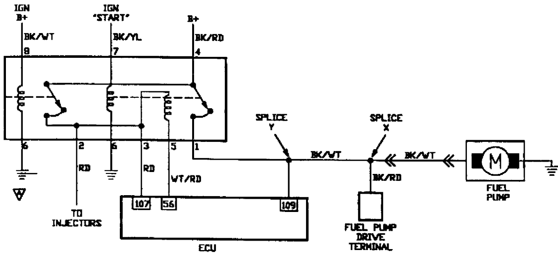
Fig. 21: No Start Test 6 Schematic Testing Control Relay
