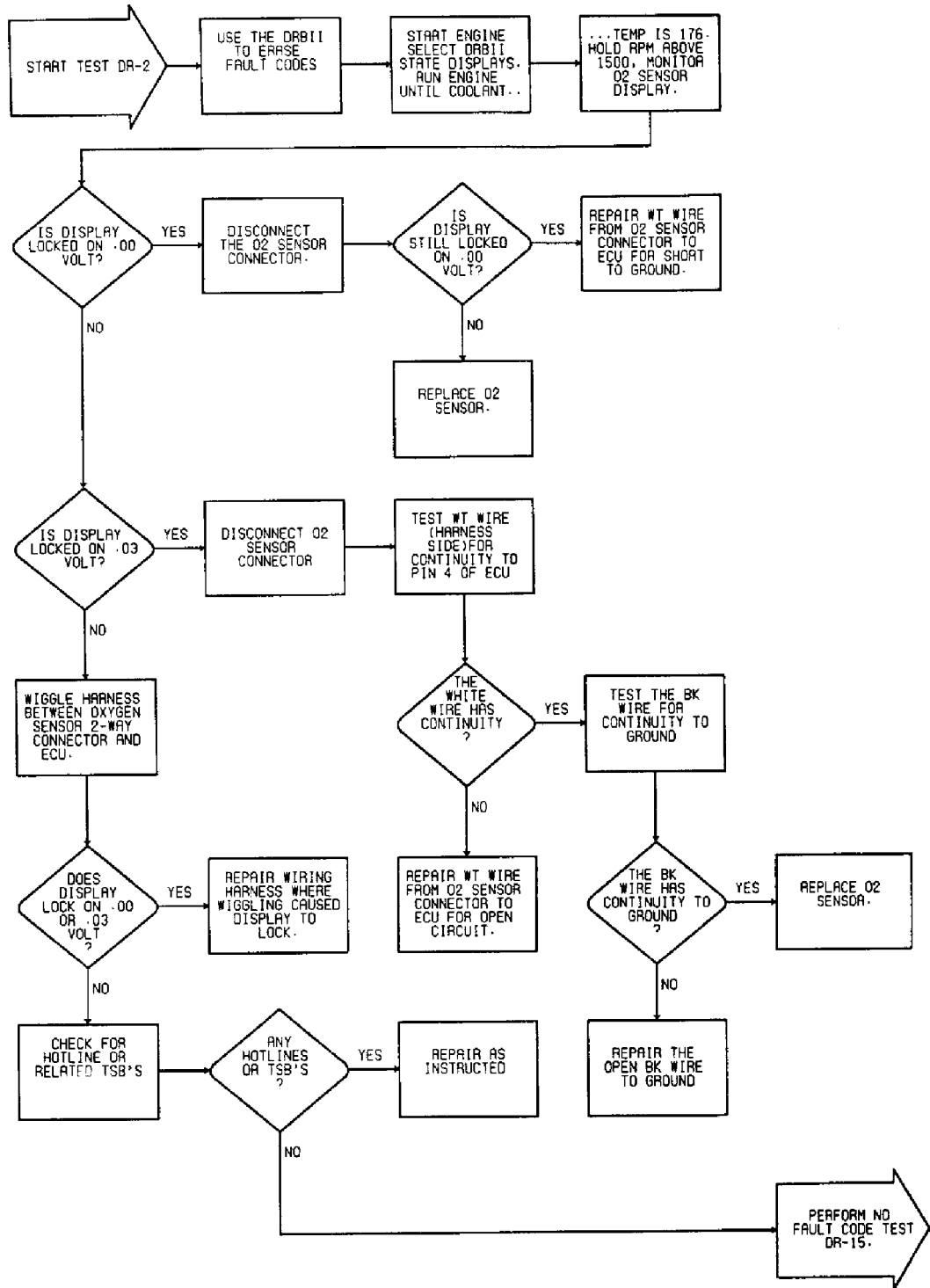
Fig. 27: DR-2 Test Flow Chart Testing Oxygen Sensor Circuit
