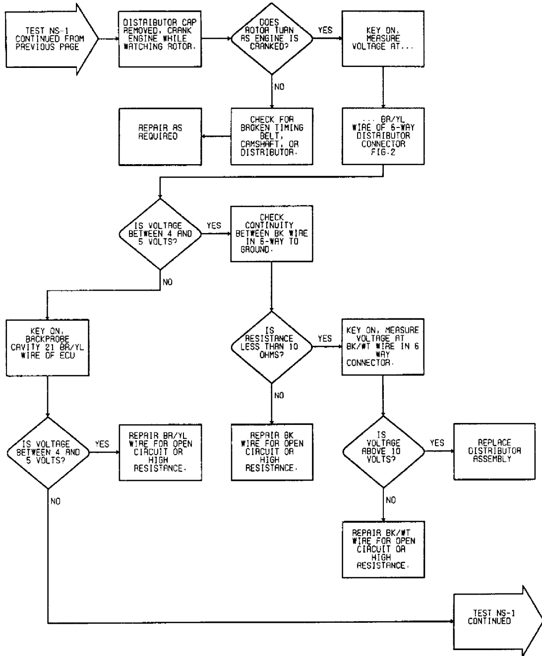
Fig. 11: No Start Test 1 Flow Chart (4 Of 5) Ignition Check
