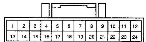
24-WAY CONNECTOR
