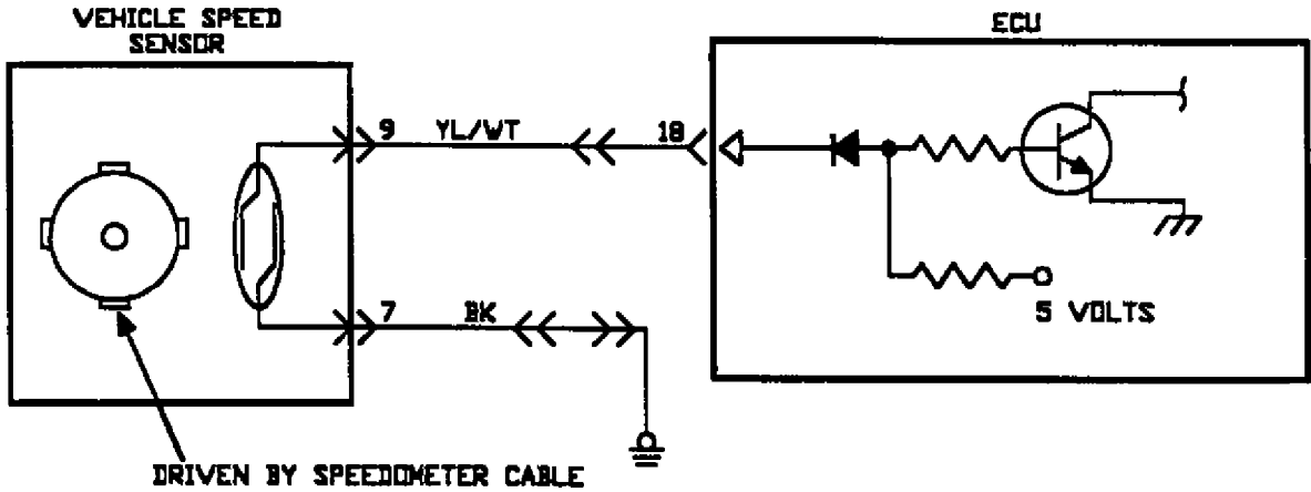
Fig. 47: DR-10 Test Schematic Testing Speed Sensor Circuit
