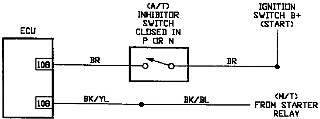
Fig. 62: DR-15 Test Schematic (1 Of 2) No Fault Code Testing
