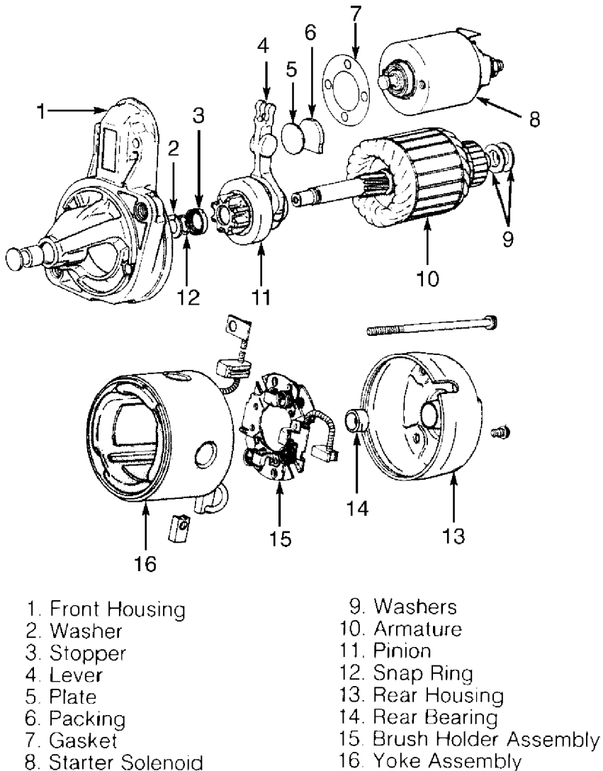
90E08772 Fig. 6: Exploded View of Direct Drive Starter Courtesy of Mitsubishi Motor Sales of America.
