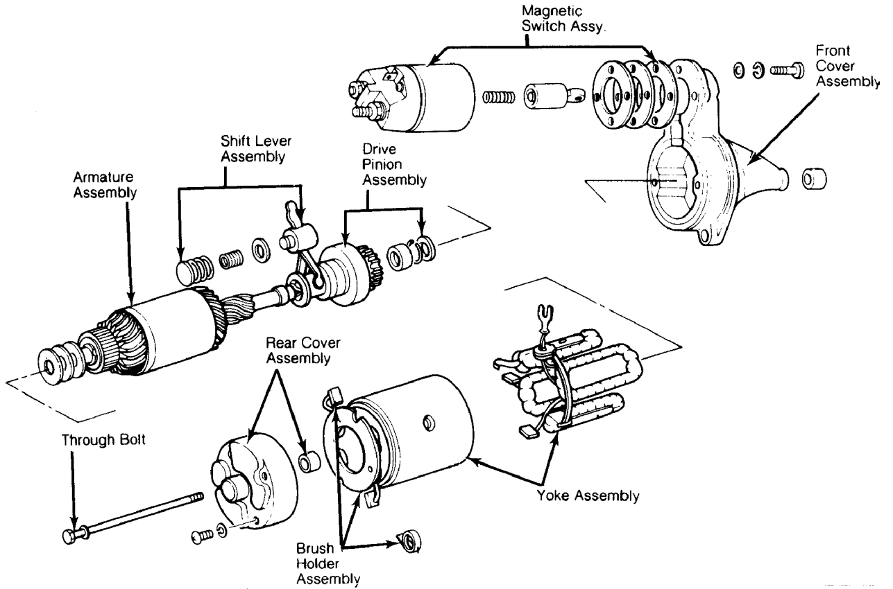
29420 Fig. 4: Disassembled View of Typical Mitsubishi Starter
